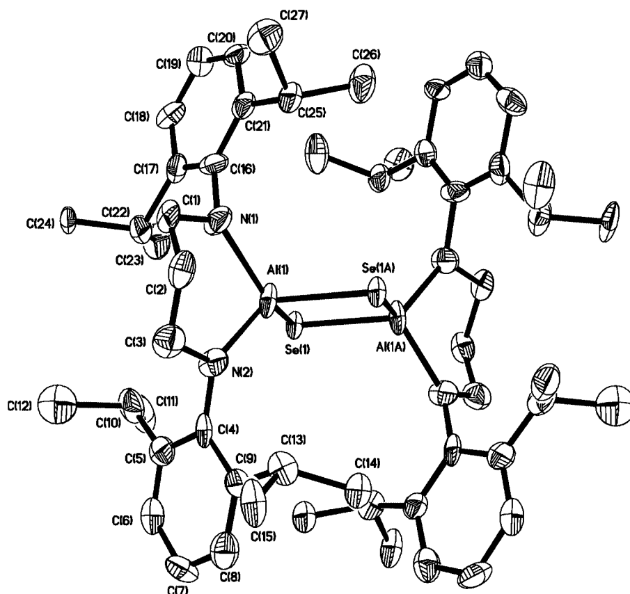
Figure 3. Molecular structure of 4 with the thermal ellipsoids at 30% probability level; H atoms are omitted for clarity
