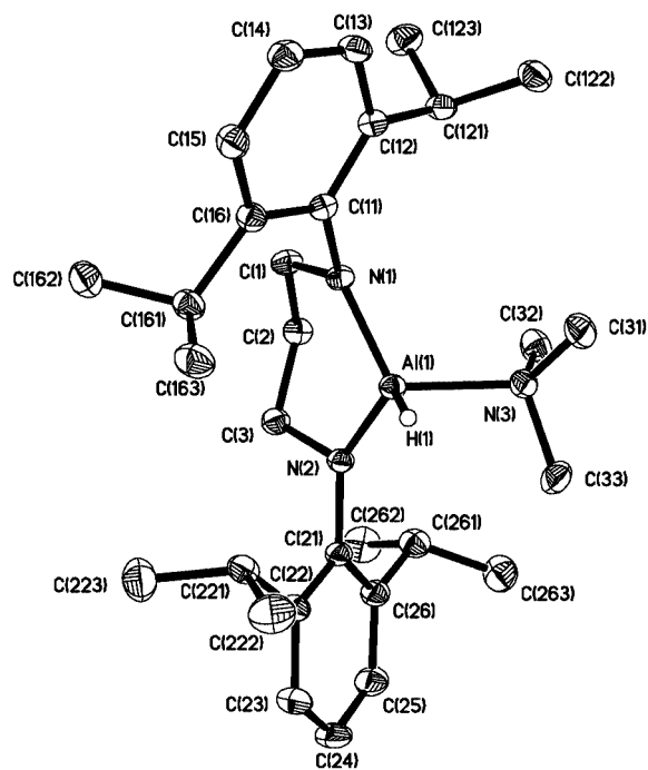
Figure 1. Molecular structure of 1 with the thermal ellipsoids at 30% probability level; H atoms are omitted for clarity except for the Al–H hydrogen atom
