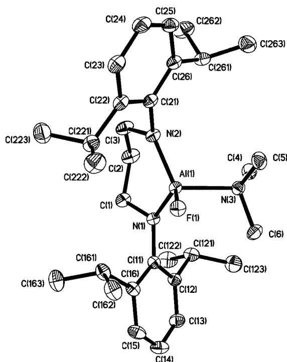
Figure 2. Molecular structure of 2 with the thermal ellipsoids at 30% probability level; H atoms are omitted for clarity
